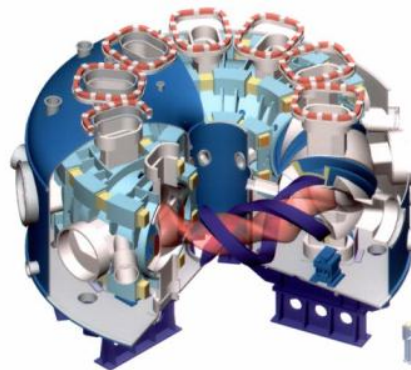
Cutaway drawing of the LHD stellarator
