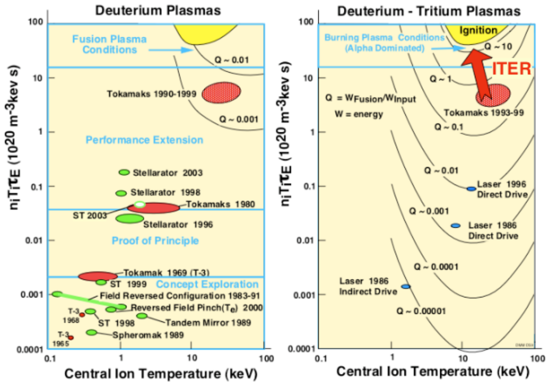
Fig. 2.b.2 Lawson Diagram for Magnetic Fusion
