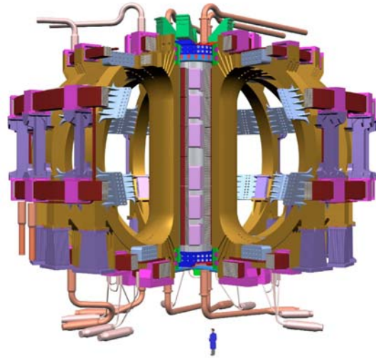
The ITER superconducting coil set
