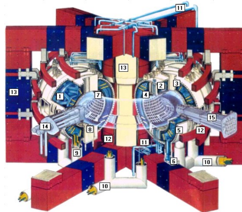
Cutaway drawing of the Tore Supra device.
