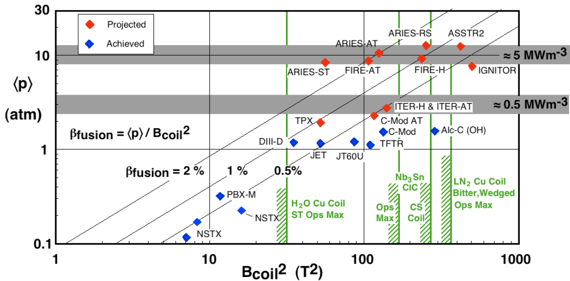
Fig. 4.b.2.2 Plasma pressure vs magnetic field at the coil.
