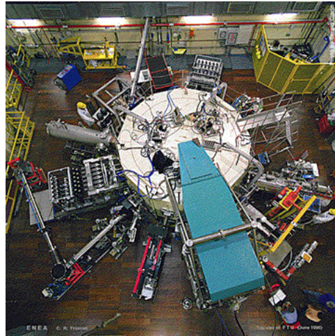
The Frascati Tokamak Upgrade
