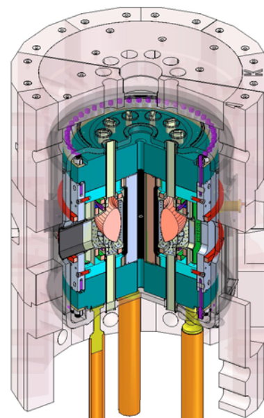
Alcator C-Mod Tokamak
