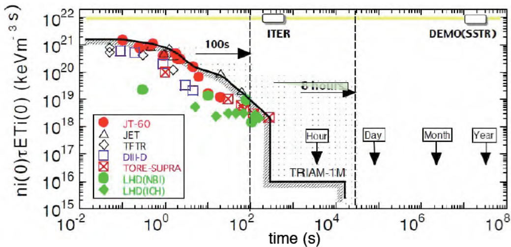
Fig. 4.b.2.1 Plasma performance vs pulse length (Kikuchi FT 2-5, 21 st IAEA Fusion Energy Conference, Chengdu, China, 2006)
