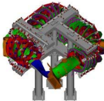
Cutaway drawing of the HSX stellarator.
