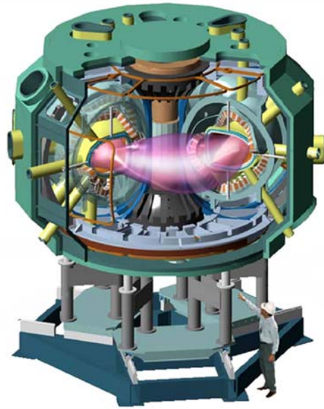
The NCSX Stellarator
