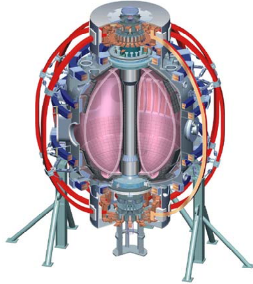
Cross-section of the NSTX device showing major device components.
