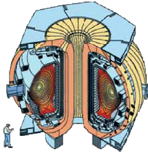
The DIII-D Tokamak
