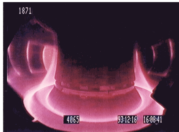
Photograph of a plasma in ASDEX-Upgrade
