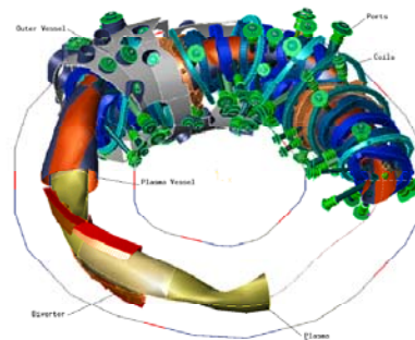
Cutaway drawing of the W7X Stellarator.
